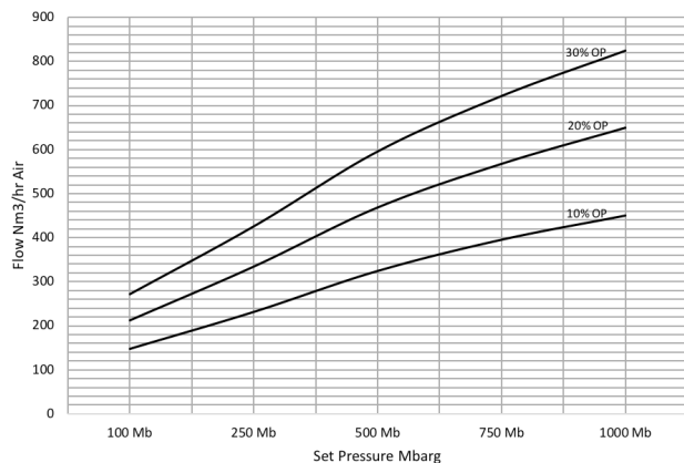
2" Pressure Flow B300 Open Spring
