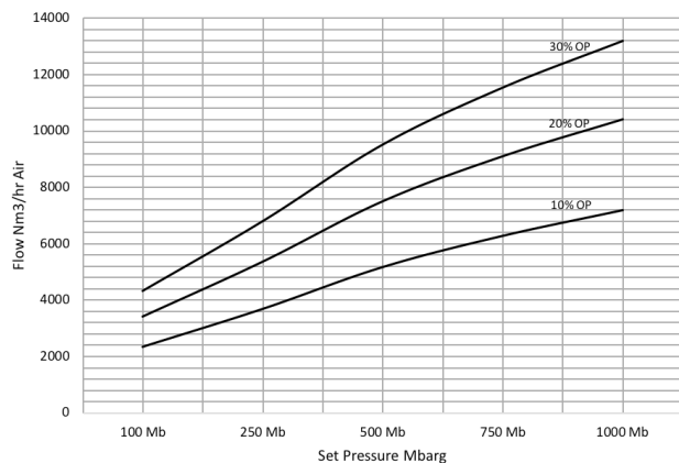
8" Pressure Flow B300 Open Spring
