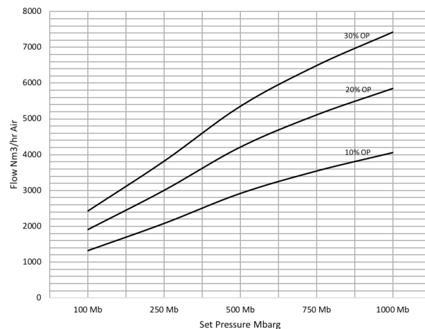
6" Pressure Flow B300 Open Spring
