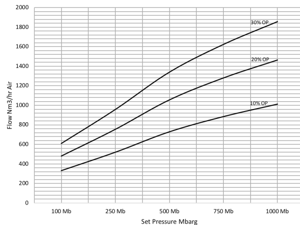
3" Pressure Flow B300 Open Spring
