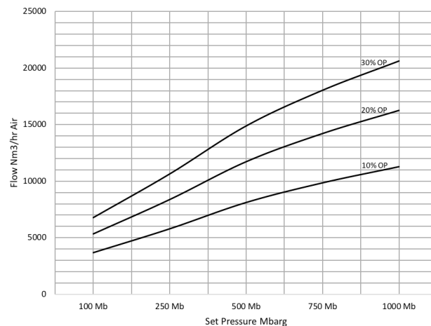
10" Pressure Flow B300 Open Spring
