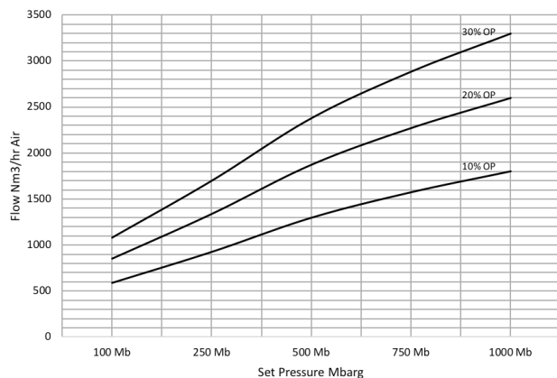
4" Pressure Flow B300 Open Spring
